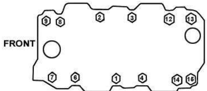
300-563 & 300-564 Torque Sequence
