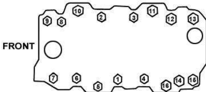
300-561 & 300-562 Torque Sequence
