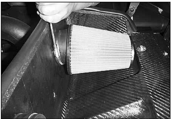
30. Install the K&N® air filter elements onto the intake tubes and secure with hose clamps.
