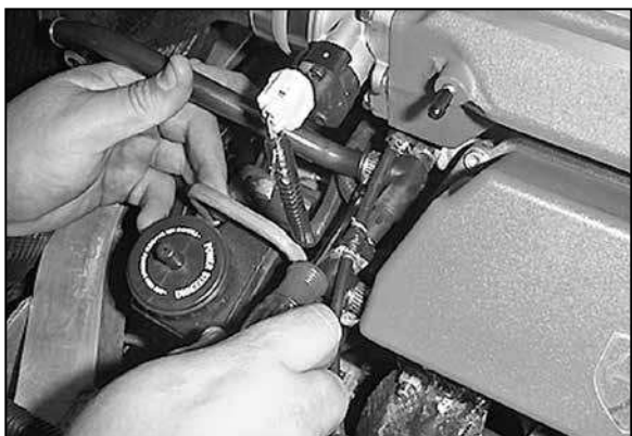
26. Reinstall the vent tube.
