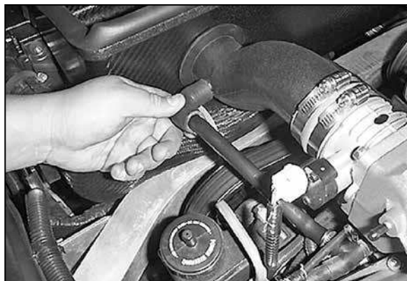
27. Using the vent hose provided, connect the vent tube to the vent on the intake tube.
