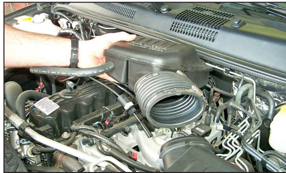
4. Loosen the hose clamp at the air cleaner lid and at the throttle body, then, remove the resonator and bellows assembly as shown.
