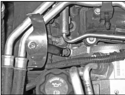
16. Install the tube mounting bracket assembly onto the A/C compressor using the bolt removed in step #14 as shown.
