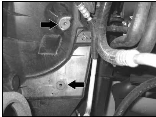
12. Install the two threaded inserts into the air box mounting grommets location as shown.
