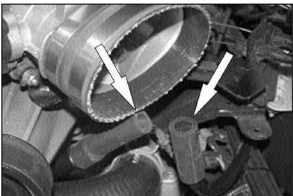
20. Install the two provide 5/8 silicone hoses onto the idle air and crank case vent lines as shown.
