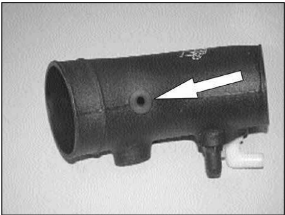
17. Install the provided grommet into the new intake tube as shown.
