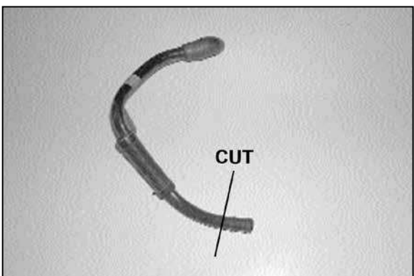
19. Cut the end off the idle air vent tube just below bead as shown. Then re-install vent tube back onto vehicle.
