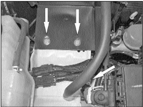
12. Install the heat shield into vehicle, then secure with the provided hardware as shown.
