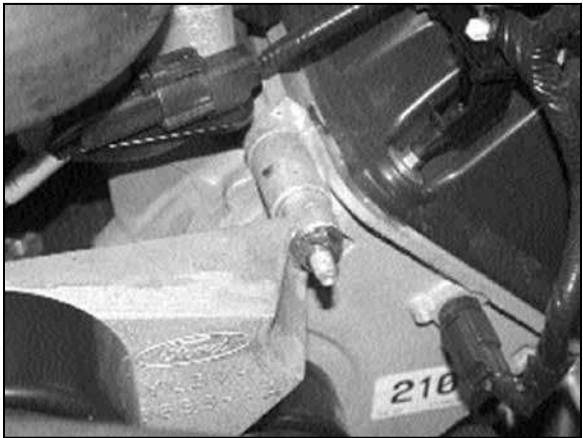
13. Remove the 8mm nut from stud that retains the idler pulley bracket.
