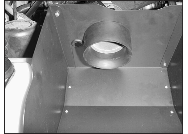
22. Install the mass air sensor into the hole on the heat shield as shown.
