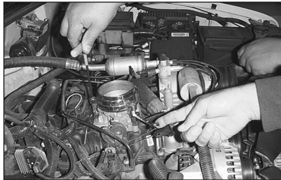
17. Using a 7/16" wrench, snug the three coupling nuts and tighten the three 6mm bolts using a 5mm allen wrench.
