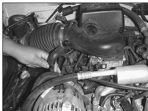
4. Disconnect the crankcase vent hose from the factory air intake tube.
