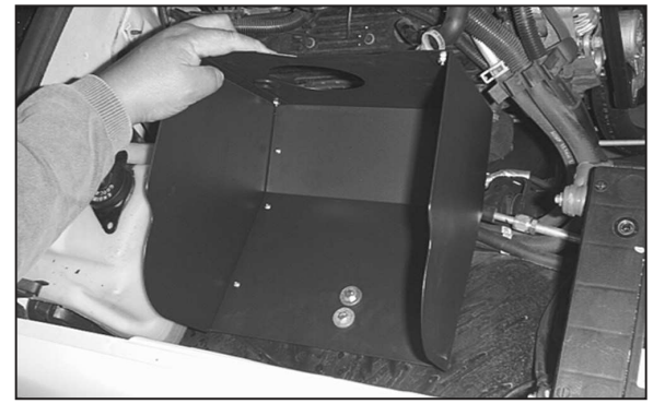
23. Install the heat shield assembly into the two holes on the inner fender and secure from underneath.
