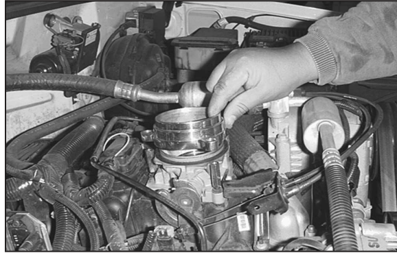
16. Install the aluminum throttle body adapter and hand start the three 6mm allen bolts.
