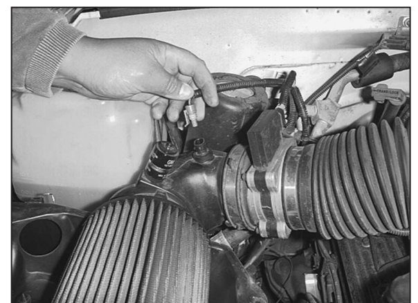
5. Disconnect the air temperature sensor electrical connection.
