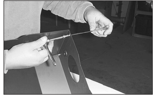
18. Using a 1/8" allen wrench and a 3/8" socket, assemble the heat shield using the provided hardware.
