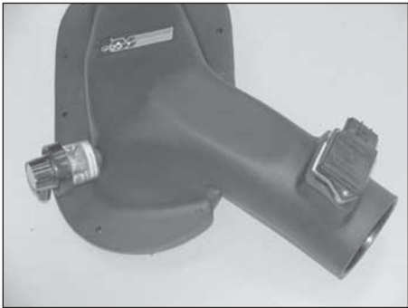
20. Install the factory grommet and restriction gauge into the K&N® air box lid as shown.
