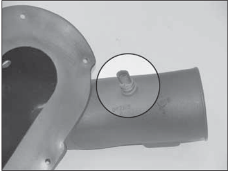
13. On vehicles equipped with the air temperature sensor, install the factory grommet and temperature sensor removed in step #11 into the K&N® intake tube at the hole drilled in step #12. NOTE: Take care when handling the temp sensor as it is very fragile.
