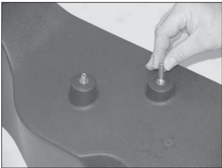
21. Install the two 8mm studs into the mounting boss on the bottom of the K&N® air box base as shown.
