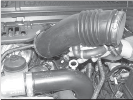
9c. On 2006 and later vehicles, remove the intake bellows and tube assembly from the vehicle as shown.
