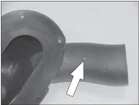
12. On vehicles equipped with an air temperature sensor, drill a 5/8" hole into the K&N® air box lid at the drill point shown.
