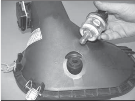
19. Remove the air filter restriction gauge and grommet from the factory air box.
