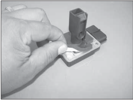
17. On vehicles equipped with a mass air sensor install the provided gasket onto the mass air sensor with the sticky side down.
