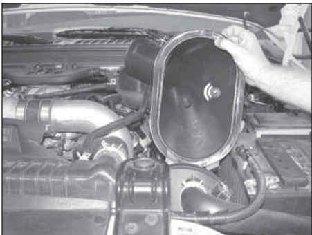
8. Remove the air box base as shown.
