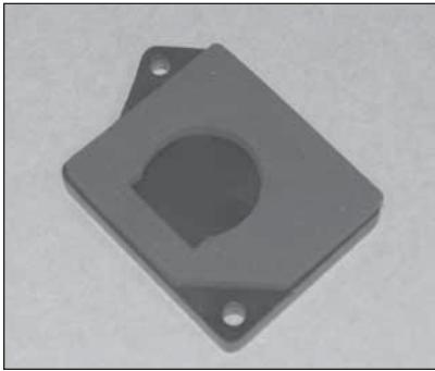
14. On vehicles equipped with an air temperature sensor, install the provided gasket onto the mass air block off plate as shown.
