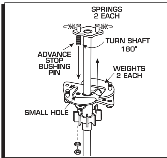
Figure 8 Locking Out the Centrifugal Advance.
