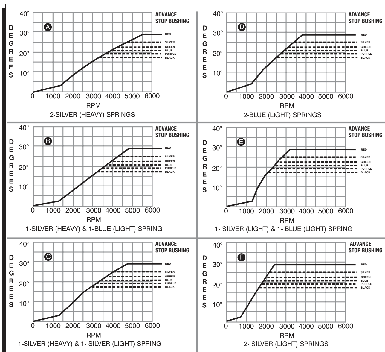
Figure 4 Advance Curves.
