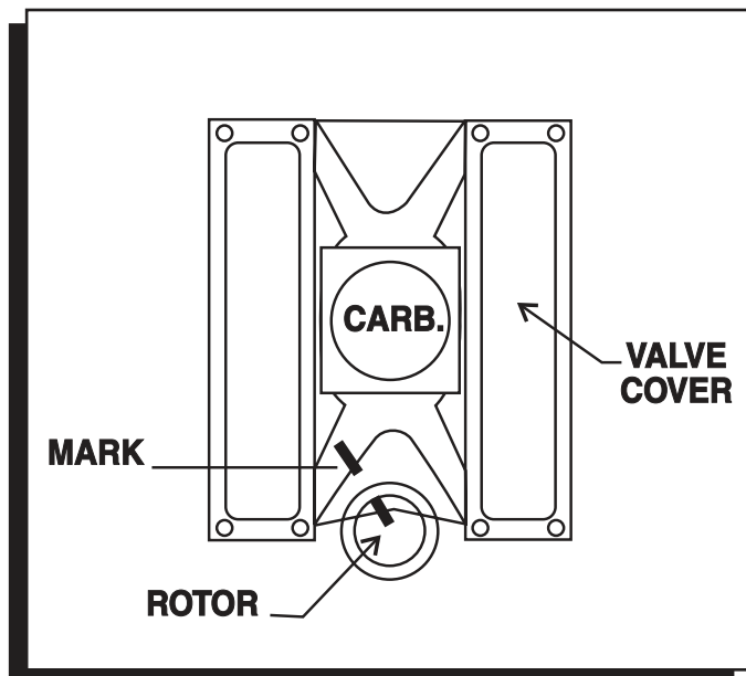
Figure 9 Marking the Rotor Location.
