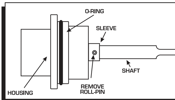
Figure 7 Removing the Retaining Sleeve.
