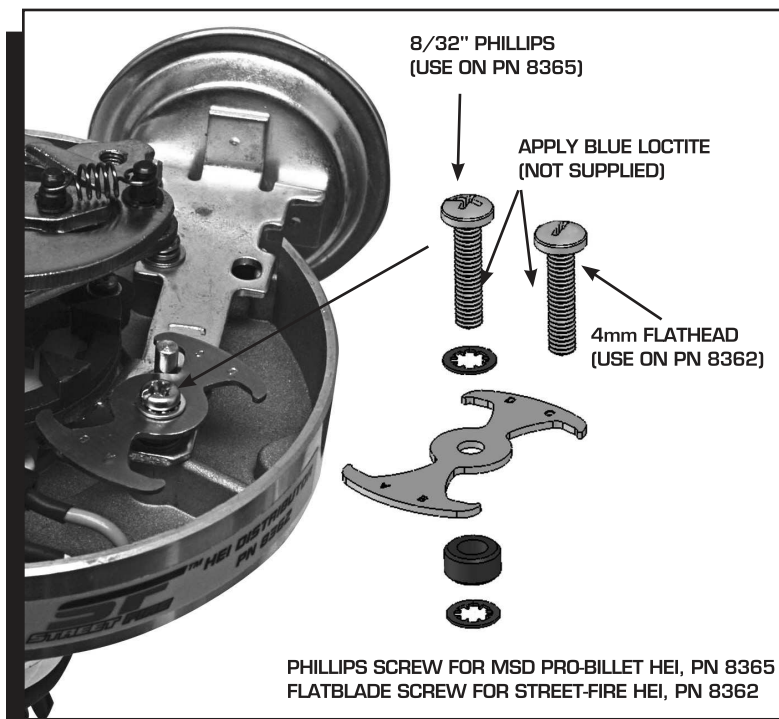
Figure 2 Installation.
