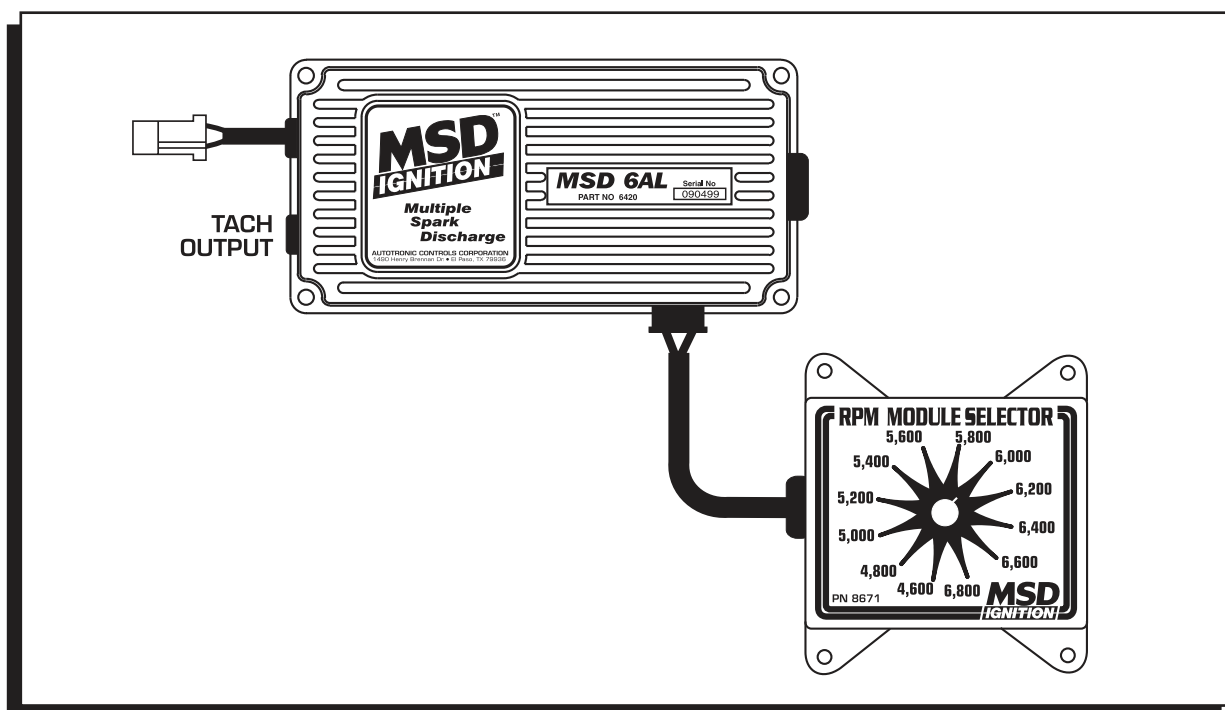
Figure 1 RPM Module Selector Installation.
