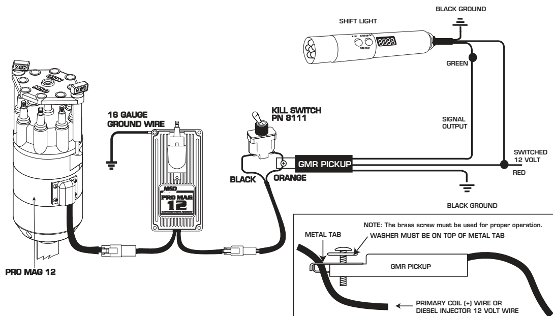
Figure 6 Wiring the 12 Amp Pro Mag.
