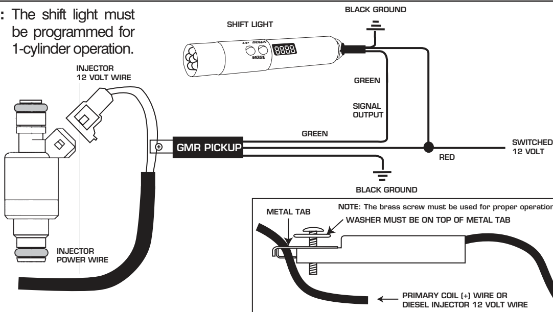
Figure 7 Installation to a Diesel Injector.
